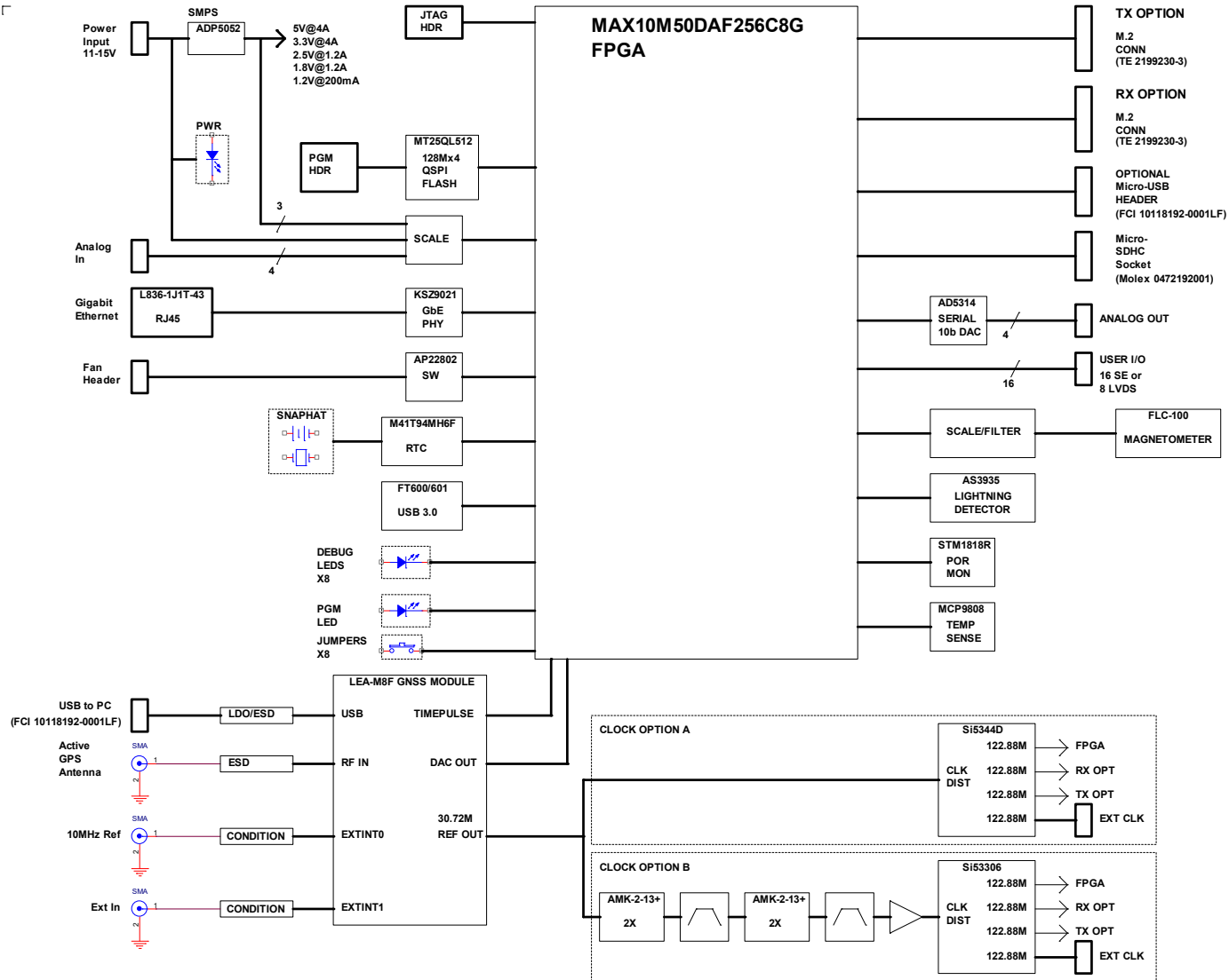
Figure 1 Data Engine Block Diagram
