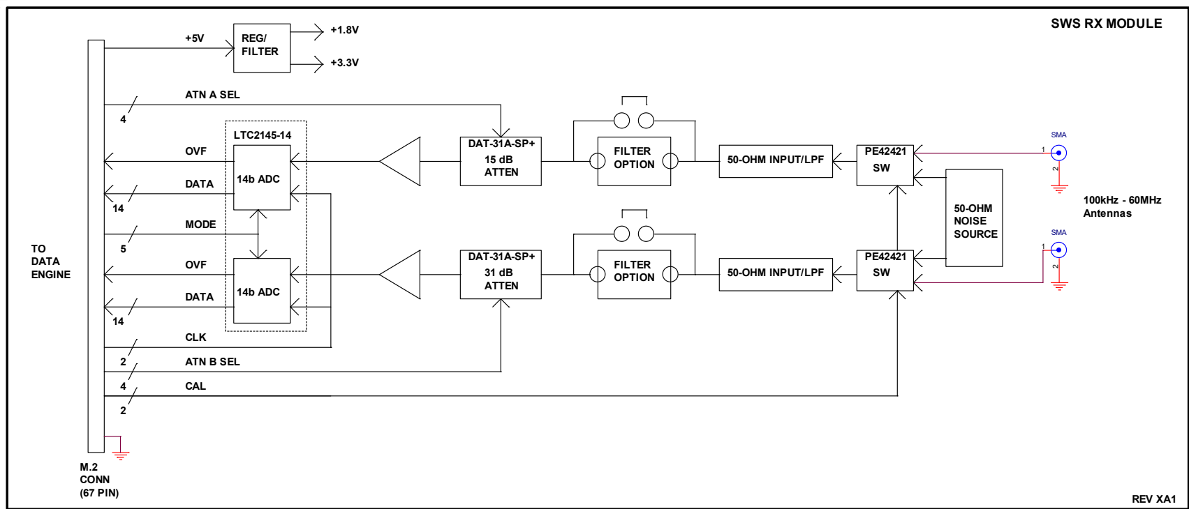
Figure 3 Space Weather Station Receiver Module
